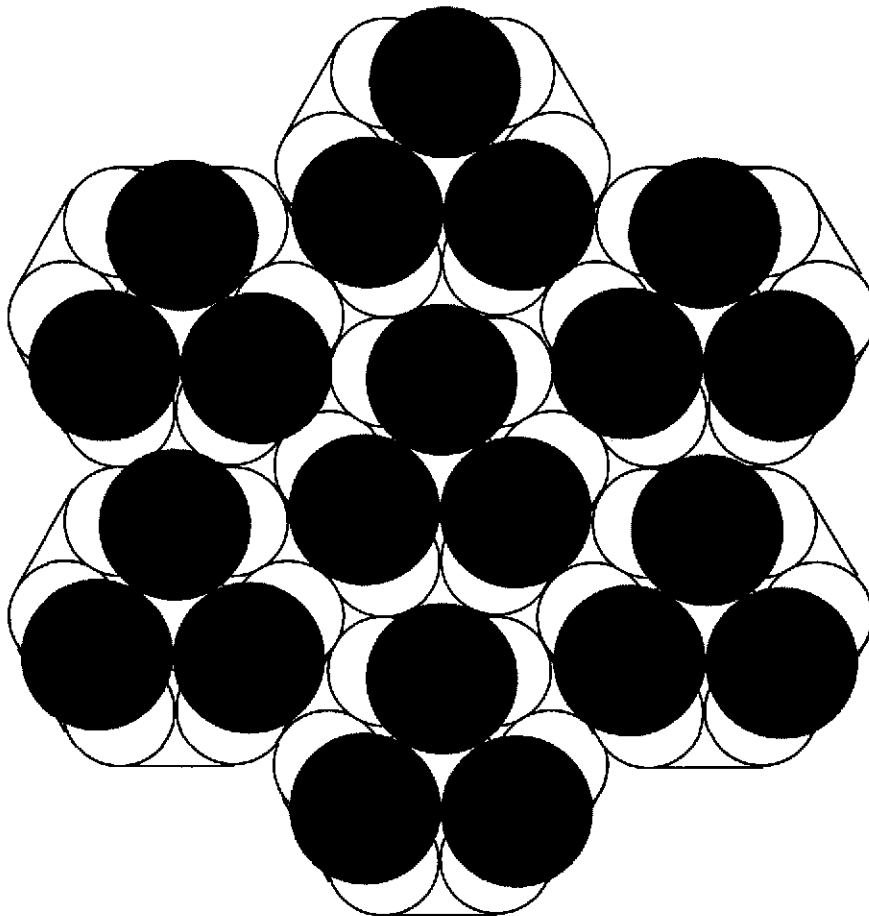
Figure 3. Schematic Diagram Showing That Three-Packs of 100-gallon Containers (Shown as Dark Circles) Fit within the Footprint of Seven-Packs of 55-gallon Drums (Shown in Outline).
