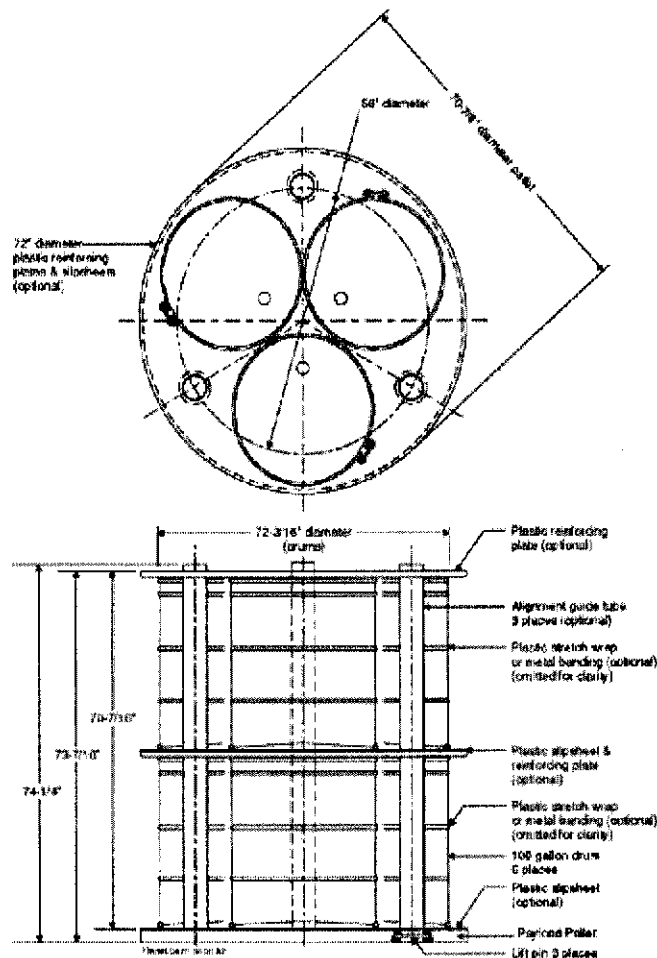
Figure 2. Six 100-Gallon Drum Payload Assembly Configuration (DOE 2000, Figure 2.1-7)
